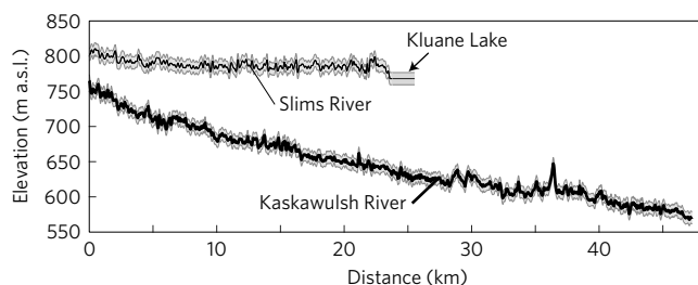
Figure 5 | Longitudinal profiles of the Slims and Kaskawulsh rivers. Elevations are derived from the 30-m ASTER GDEM v2 and smoothed using a 5-bin moving average filter. The grey error envelope represents the published root mean square error (RMSE) of \sim 8.7 m (ref. 29). The absolute vertical accuracy is 17 m. Profile locations are shown as solid yellow lines in Fig. 1.
